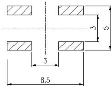
P. C. Board Dimension
